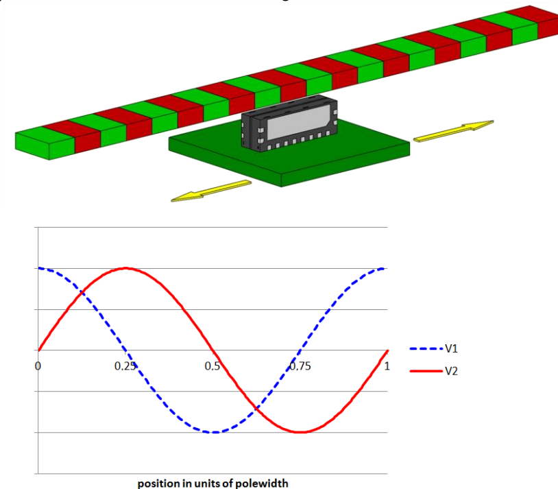
Figure 2: Typical application of a PCB mounted KMXPn002 sensor moving relative to a magnetic pole and the corresponding output signal voltage depending on sensor position
