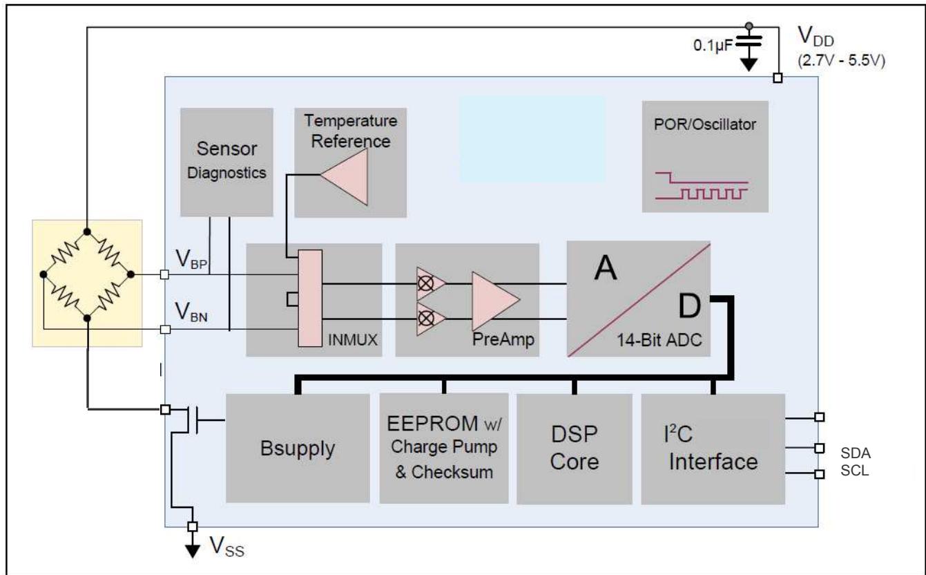
Block Diagram – I 2 C Digital Output (Digital)
