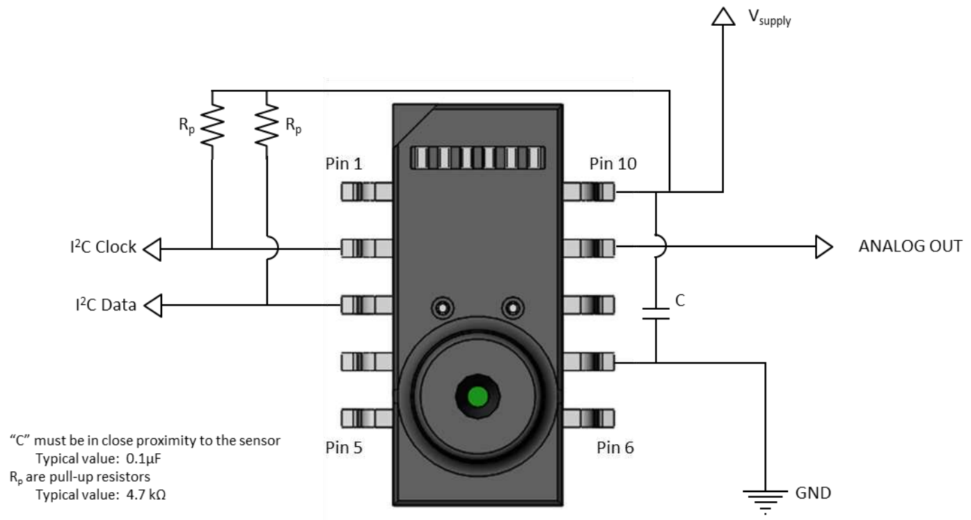
Applications Circuit for SOIC-10 Package
